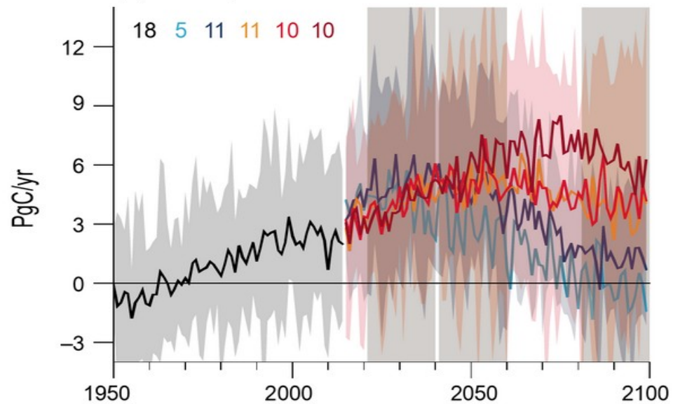
(b) Atmosphere to land carbon flux
