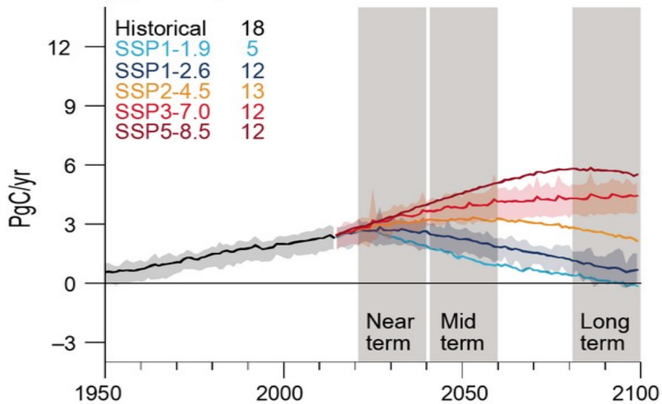
(a) Atmosphere to ocean carbon flux
