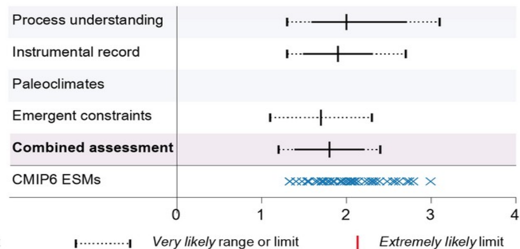
(b) Transient climate response estimates (°C)
