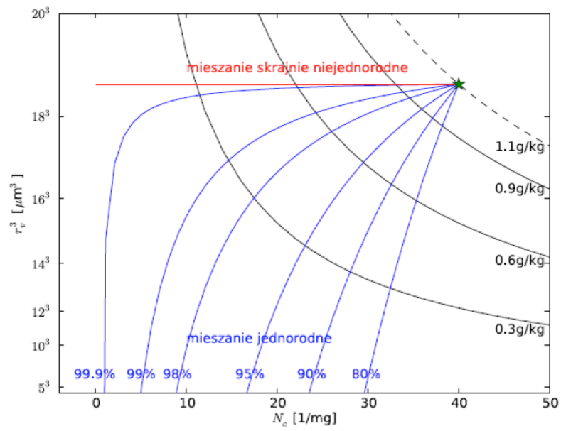
Figure 1: Entrainment diagram. Mieszanie skrajnie niejednorodne means Extremely inhomogeneous mixing , Mieszanie jednorodne means Homogeneous mixing .
