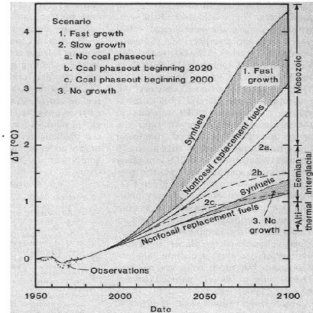
Fig. 6. Projections of global temperature. The diffusion coefficient beneath the ocean mixed layer is 1.2 \text{ cm}^2 \text{ sec}^{-1} , as required for best fit of the model and observations for the period 1880 to 1978. Estimated global mean warming in earlier warm periods is indicated on the right.
