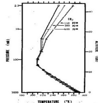
FIG. 16. Vertical distributions of temperature in radiative-convective equilibrium for various values of \text{CO}_2 content.
