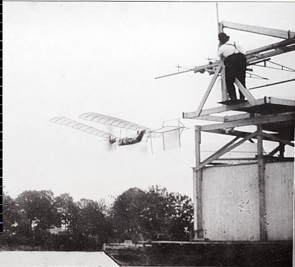
INSTANTANEOUS PHOTOGRAPH OF THE AERODROME AT THE MOMENT AFTER LAUNCHING IN ITS FLIGHT AT QUANTICO ON THE POTOMAC RIVER, MAY 6, 1896. ENLARGED TEN TIMES
