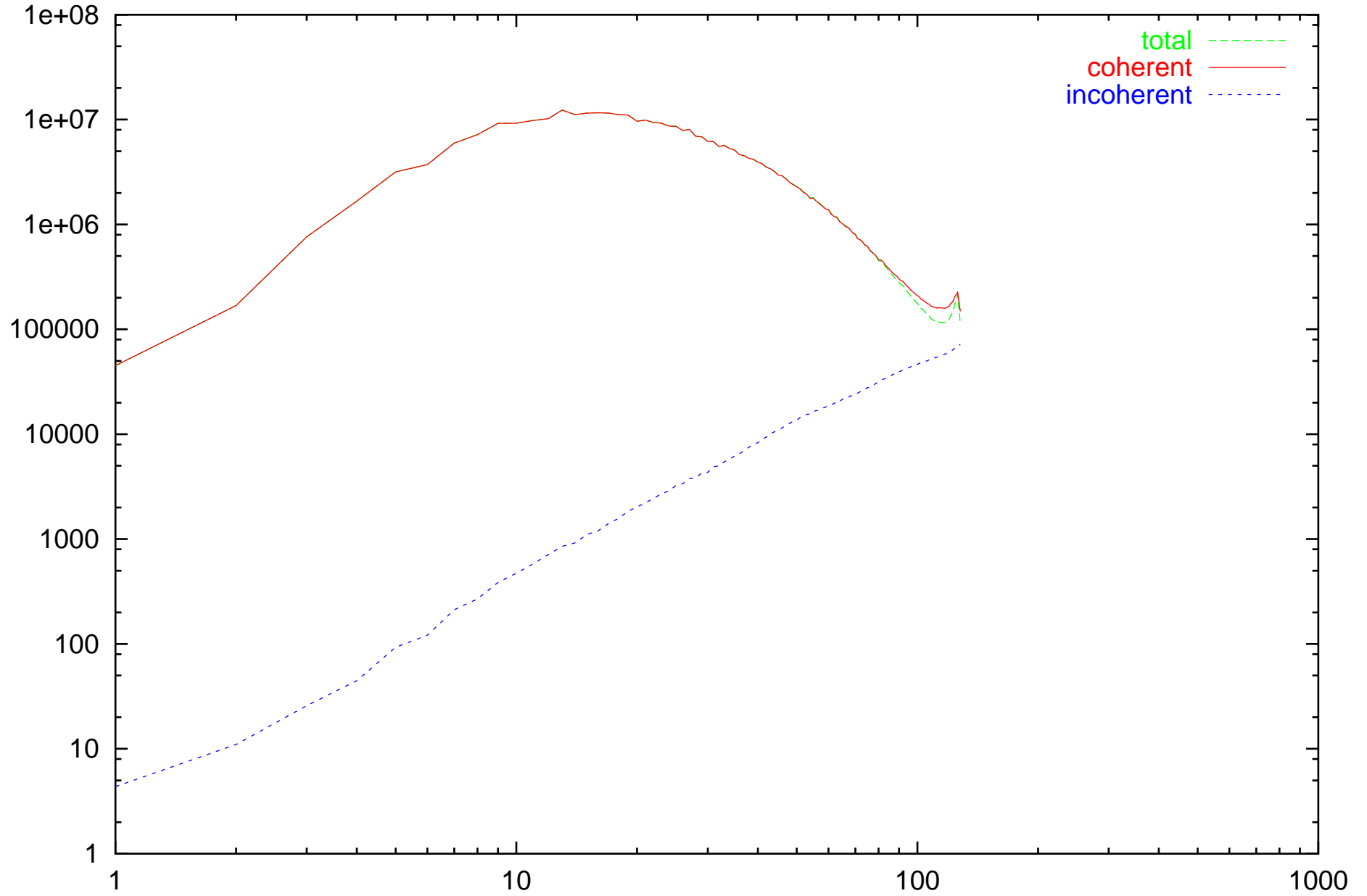
Potential Enstrophy Spectrum
