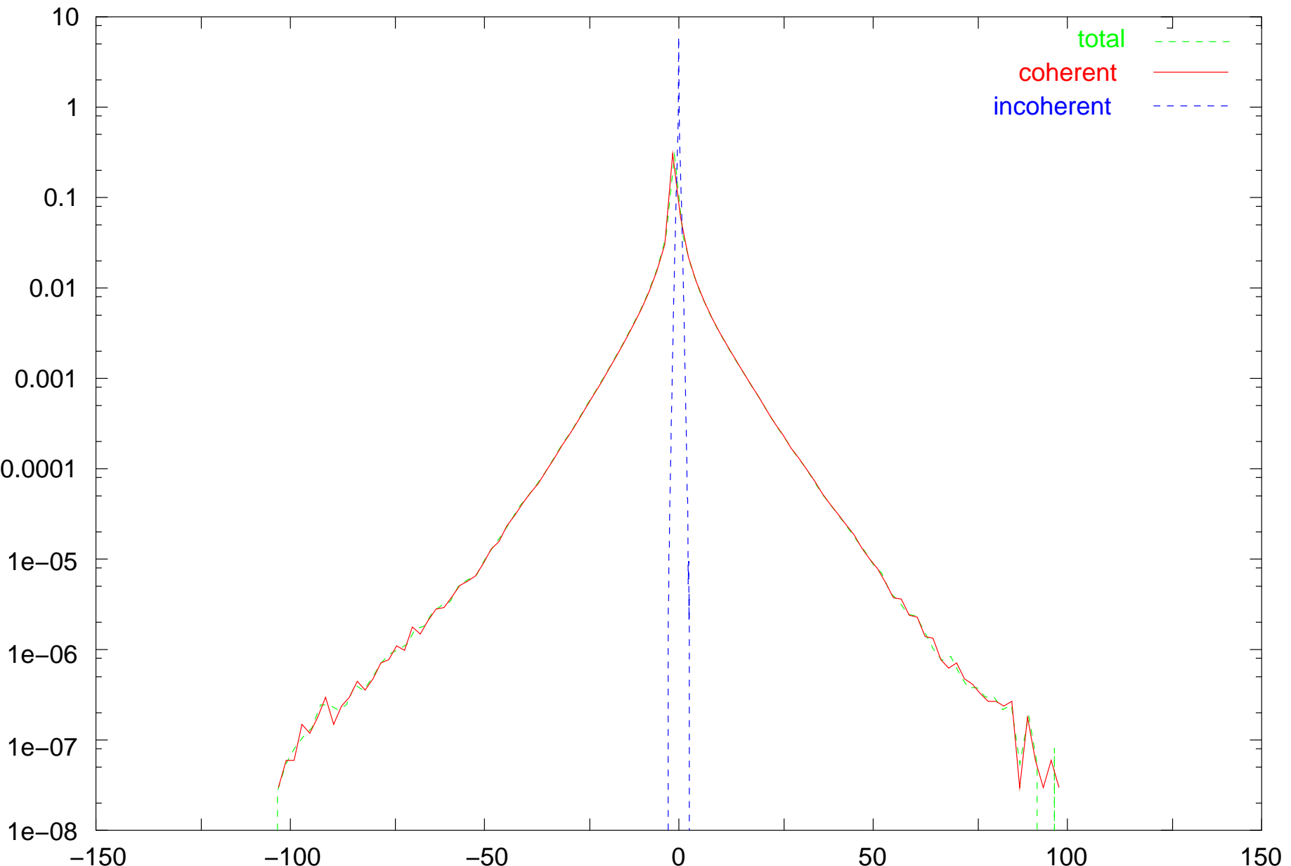
Potential vorticity
